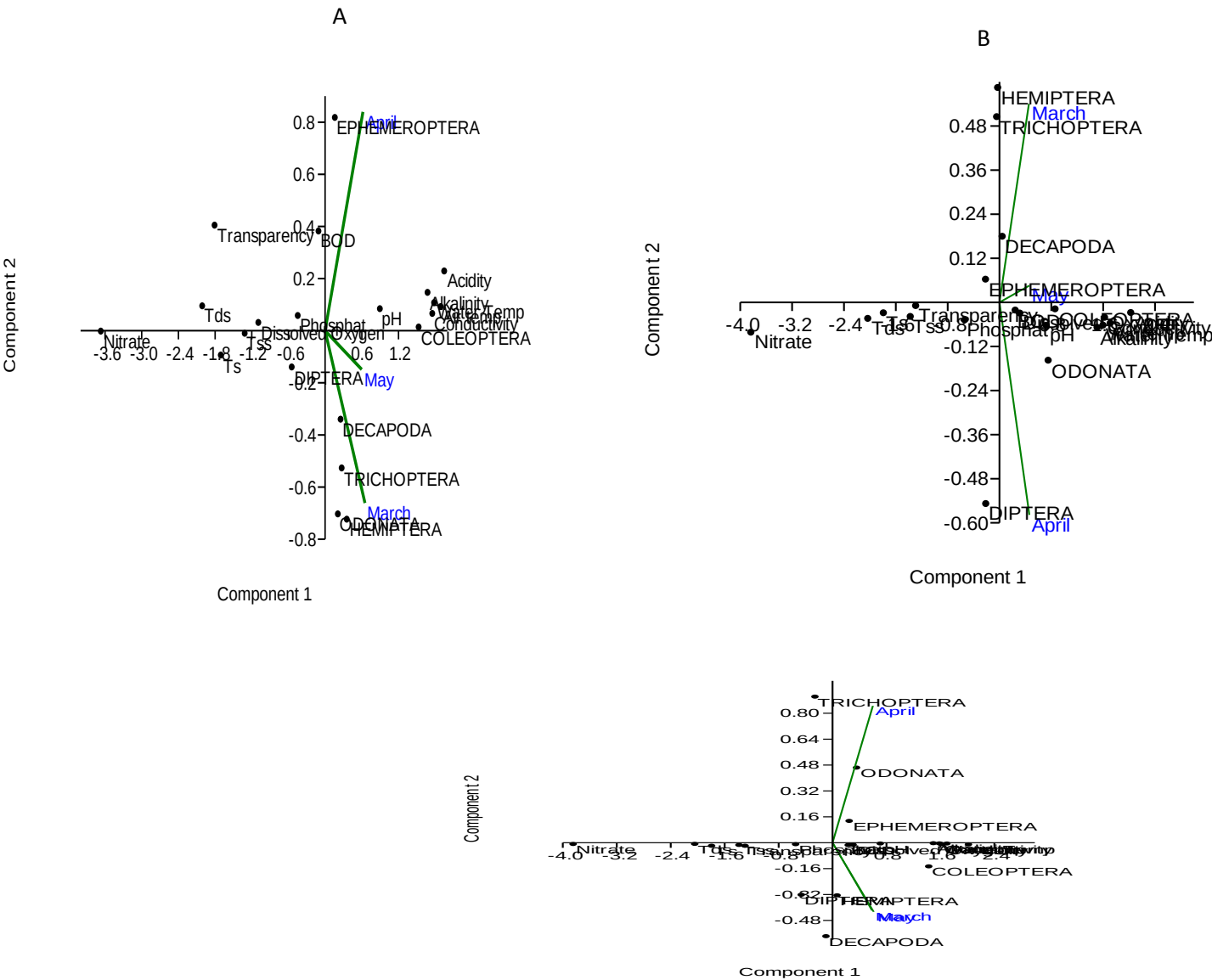
Figure 4: Principal Component Analysis (PCA) Plot of the first two principal components of the environmental variables and macroinvertebrates in Stations 1(A), 2(B) and 3(C)
