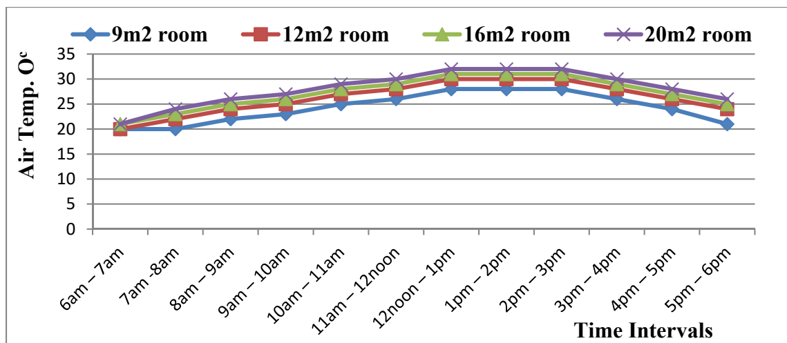
Model 5: Air Temperature of WWR 5s for 9m², 12m², 16m² & 20m²
