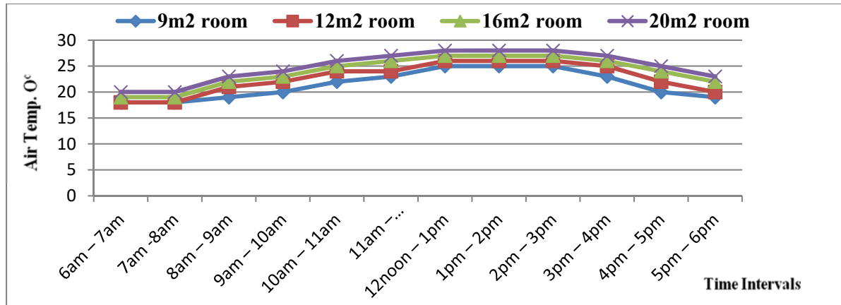
Model 4: Air Temperature of WWR 4 for 9m², 12m², 16m² & 20m²
