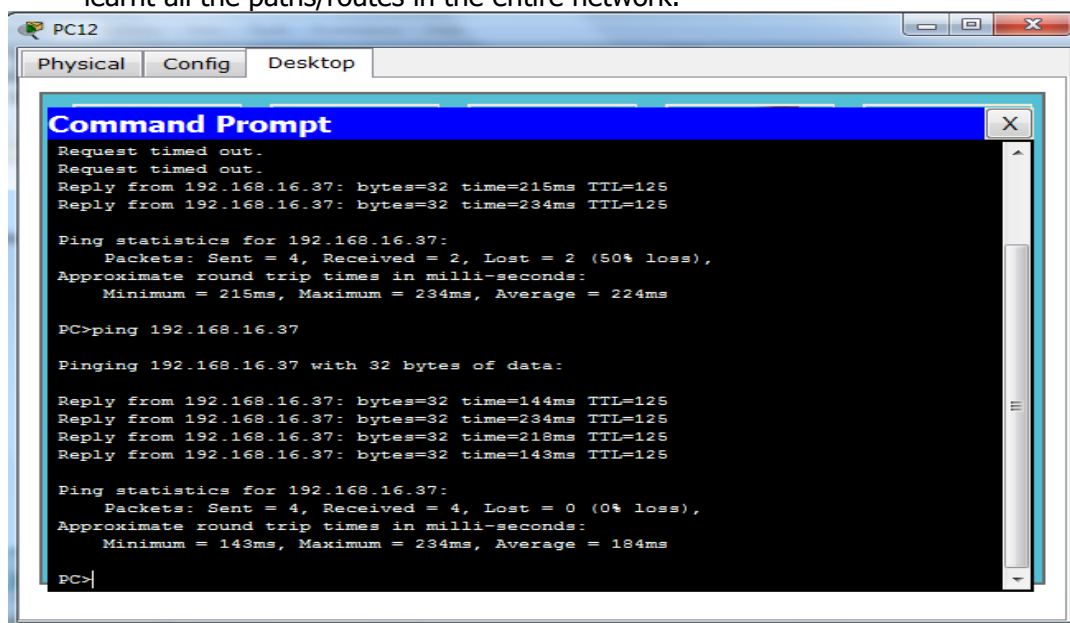
Figure 5: Screenshot Showing Connectivity from an End Device in Branch1 Network to an End Device in Branch2
