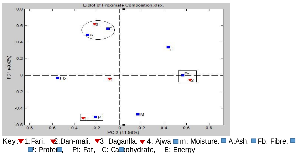
Figure 1: PCA biplot for the Proximate Composition
