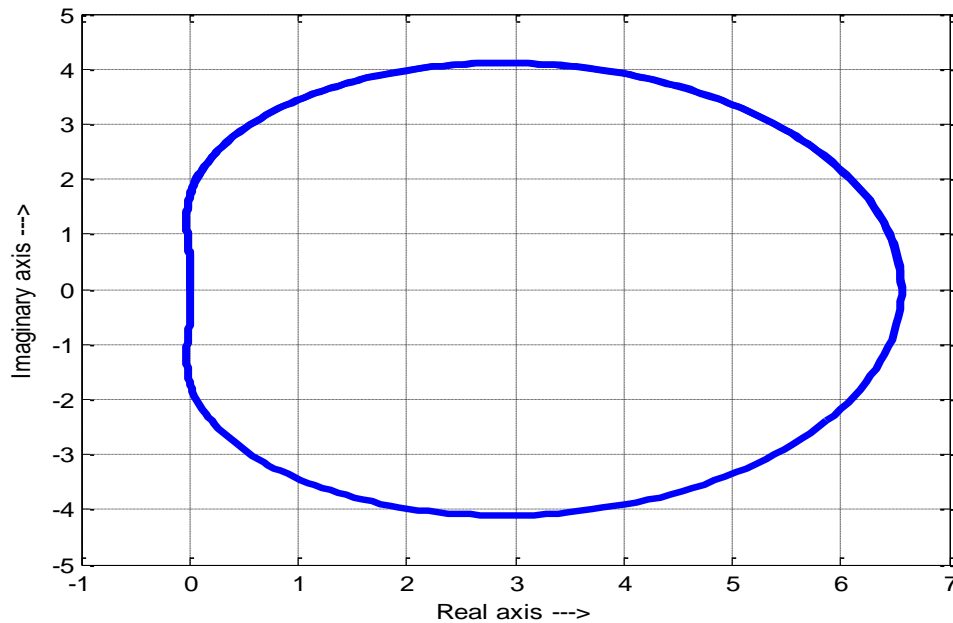
Figure 4.1: Showing Region of Absolute Stability of the HBDF
