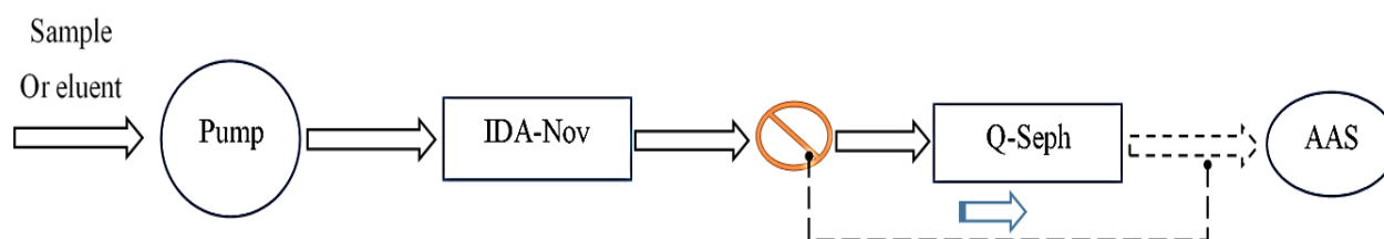
Figure 4: Online preconcentration of Cr(III) and Cr(VI) species by dual columns combined with AAS. Source: Hashemi et al. (2004)
