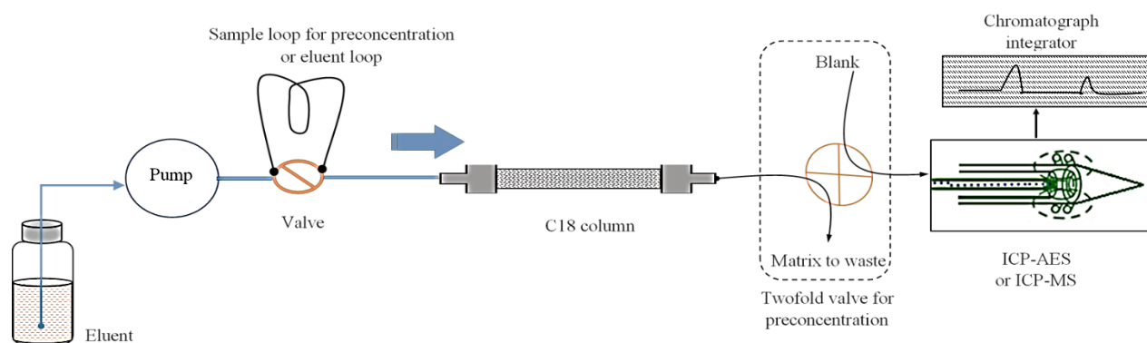
Figure 5: Schematic diagram of the online separation and preconcentration of Cr species hyphenated to ICP-MS/AES. Source: Posta et al. (1996)
