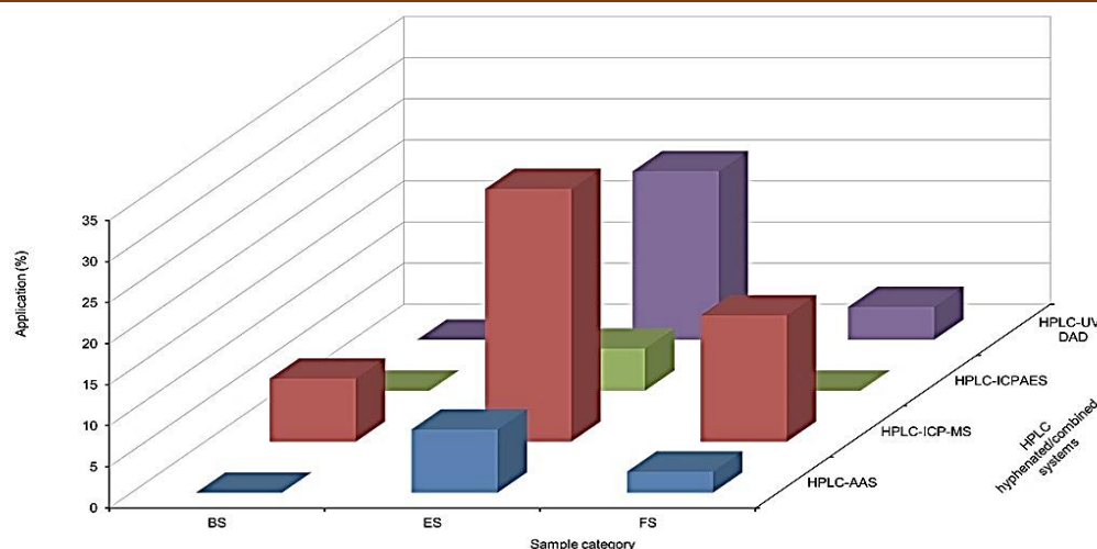
Figure 2: Sample categories used by the HPLC hyphenated systems for the speciation analysis of Cr. BS (Bio-samples), ES (Environmental samples), and FS (Food samples)
