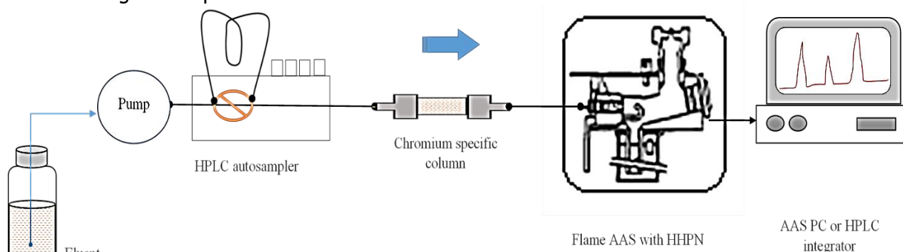
Figure 3: Set up for the online preconcentration and detection of Cr(III) and Cr(VI) species by AAS. Source: Posta et al. (1993)
