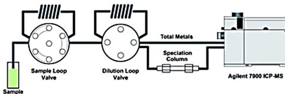
Figure 6: Fully automated total metals and chromium speciation single platform introduction system for ICP-MS. Source : (Quarles et al., 2019)
