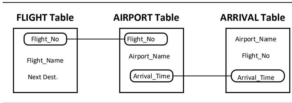
Fig. 2: A 3-way relational join.
