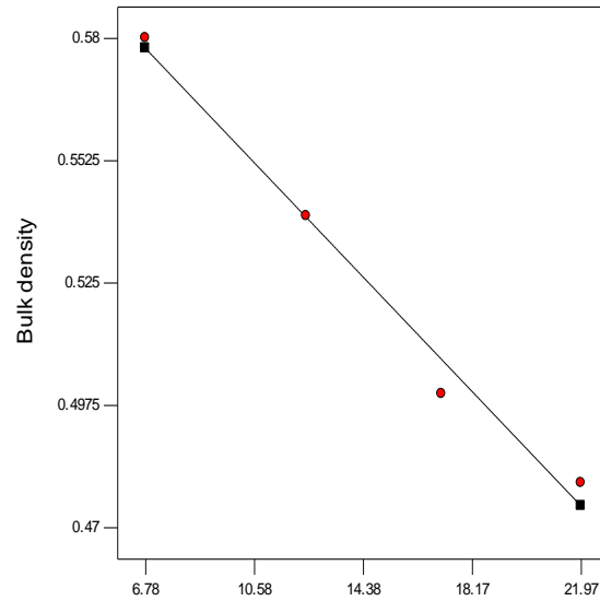
Fig. 8: Effect of Moisture content on Bulk Density
