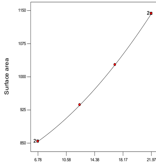
A: Moisture content Fig. 6: Effect of Moisture content on Surface Area
