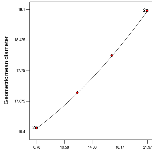
Fig. 4: Effect of Moisture content on Geometric Mean Diameter
