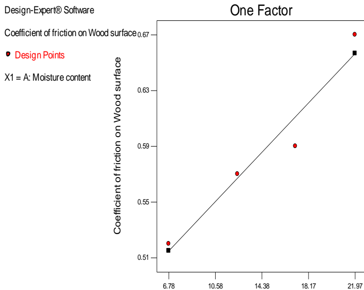
Fig. 11: Effect of Moisture content on Wooden Surface
