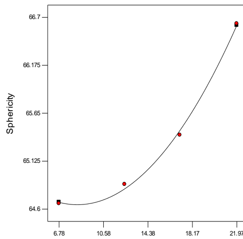
A: Moisture content Fig. 7: Effect of Moisture content on Sphericity
