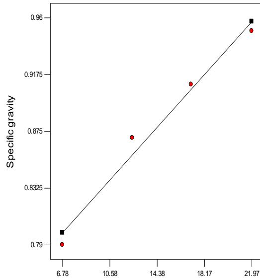
Fig. 10: Effect of Moisture content on Specific Gravity
