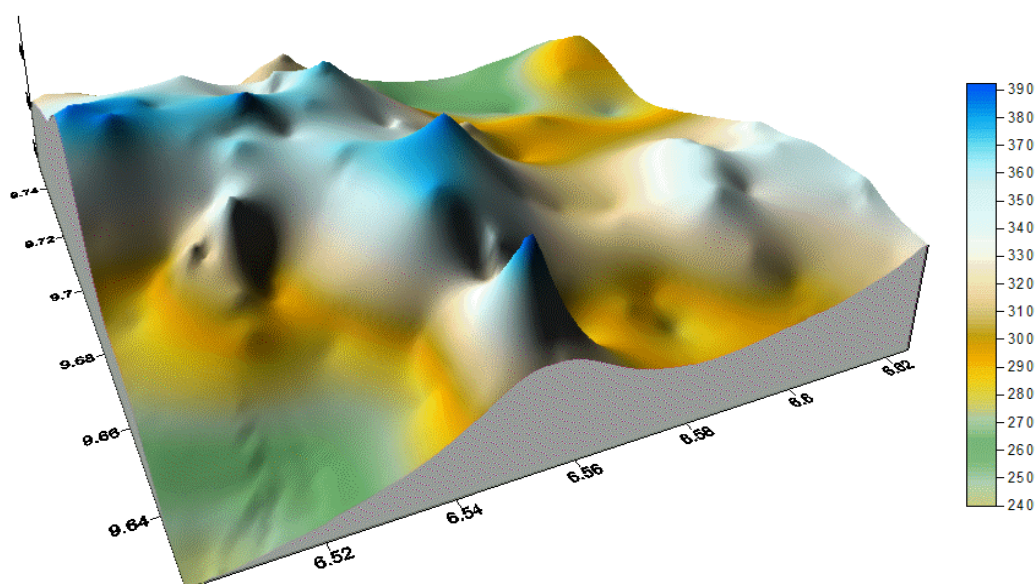
Fig. 1: Digital elevation model of the study area (Source Authors Analysis)
